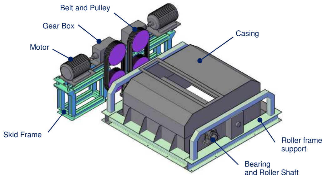
Double Roll Crusher Model
